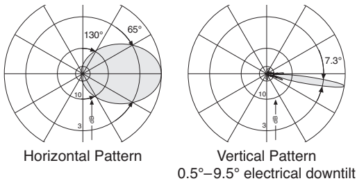
824 – 894 MHz: +45°/–45° Polarization
