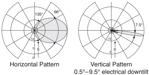
790 – 862 MHz: +45°/–45° Polarization
